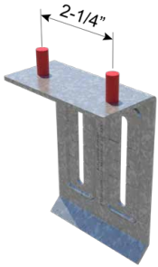
FTC3 (2) Anchor Condition
